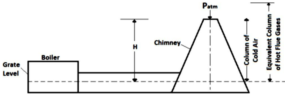
Natural Draught
