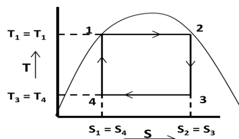
(T-s diagram)
